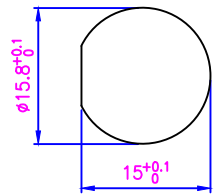
Dimensions of panel openings
